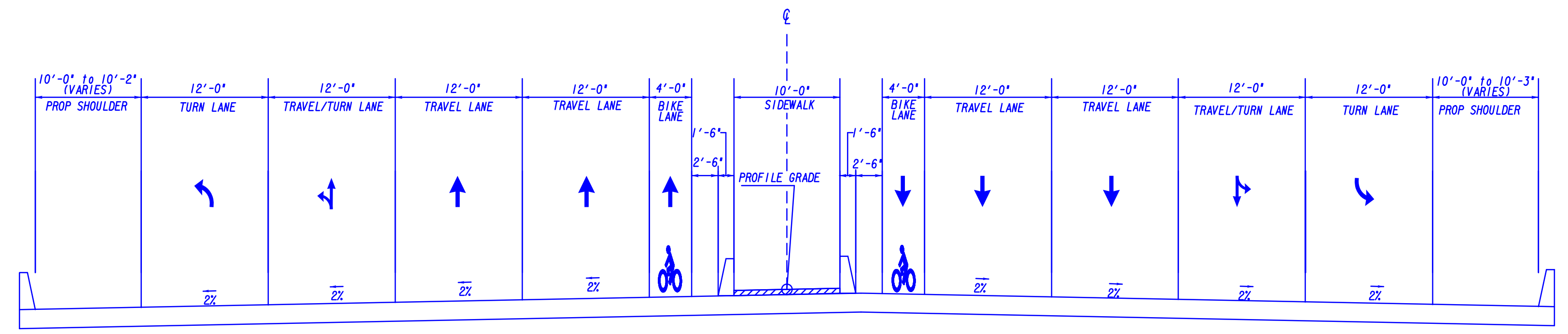
TYPICAL SECTION PANOLA ROAD TRAVELING NORTHBOUND DDI BRIDGE OVER I-20
